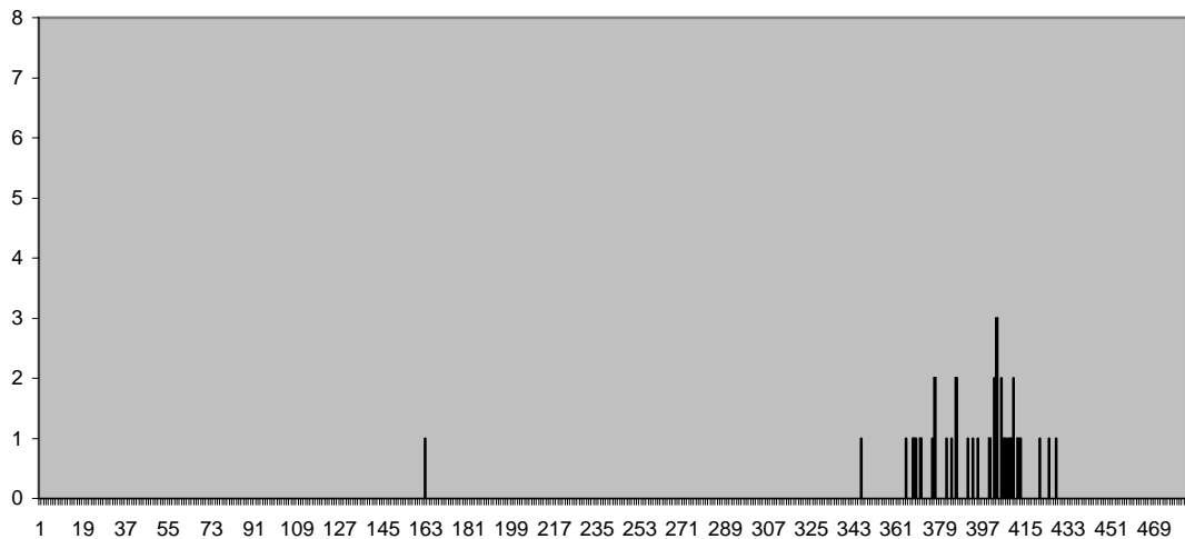
PHYS213 Scores
